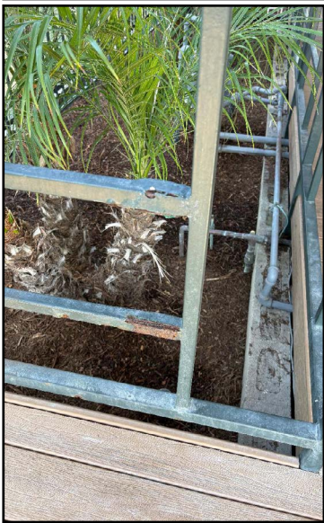
Pictured above is some wrought iron rails around the Adult Clubhouse deck that needed common repairs due to water damage by the sprinklers.
